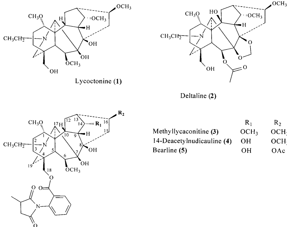
Figure 1. Chemical structures of lycoctonine (1), deltaline (2), methyllycaconitine (3), 14-deacetylnudicauline (4), and bearline (5).
