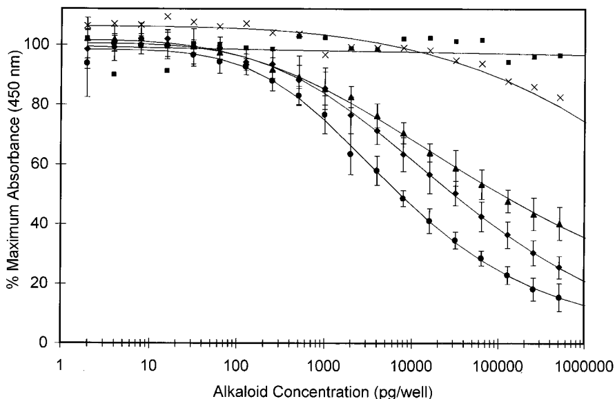
Figure 4. Inhibition curves for Assay 2. Lycoctonine ( \times ), deltaline ( \blacksquare ), methyllycaconitine ( \bullet ), 14-deacetylnudicauline ( \blacklozenge ), and bearline ( \blacktriangle ). For 14-deacetylnudicauline, methyllycaconitine, and bearline each point is the average of 9, 8, and 6 replicates, respectively. The lycoctonine and deltaline points are the average of 2 replicates.
