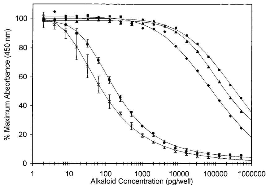
Figure 3. Inhibition curves for Assay 1. Lycoctonine ( \times ), deltaline ( \blacksquare ), methyllycaconitine ( \bullet ), 14-deacetylnudicauline ( \blacklozenge ), and bearline ( \blacktriangle ). For lycoctonine and methyllycaconitine each point is the average of 8 and 6 replicates, respectively. The 14-deacetylnudicauline, bearline, and deltaline points are the average of 2 replicates.
