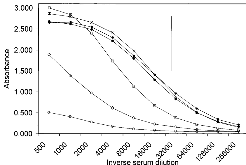
Figure 2. Titration curves for antisera-coating conjugate combinations. Antisera from sheep immunized with LYC-CDI-FET (*), LYC-SA-FET ( \square ), 14-DAN-SA-FET ( \blacklozenge ), and MLA-SA-FET ( \bullet ), 14-DAN-CDI-FET ( \circ ) with their corresponding BSA coatings. Antisera from sheep immunized with LYC-CDI-FET and with the LYC-SA-BSA coating ( \diamond ).
