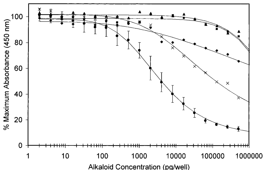
Figure 5. Inhibition curves for Assay 3. Lycoctonine (×), deltaline (■), methyllycaconitine (●), 14-deacetylnudicauline (◆), and bearline (▲). For methyllycaconitine and 14-deacetylnudicauline each point is the average of 12 and 6 replicates, respectively. The lycoctonine, deltaline, and bearline points are the average of 2 replicates.
